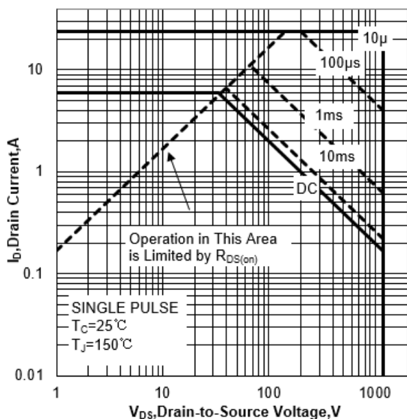
Figure 1a Safe Operating Area (No FullPAK)
